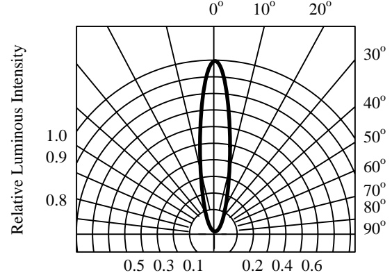
Fig 6. RADIATION DIAGRAM
